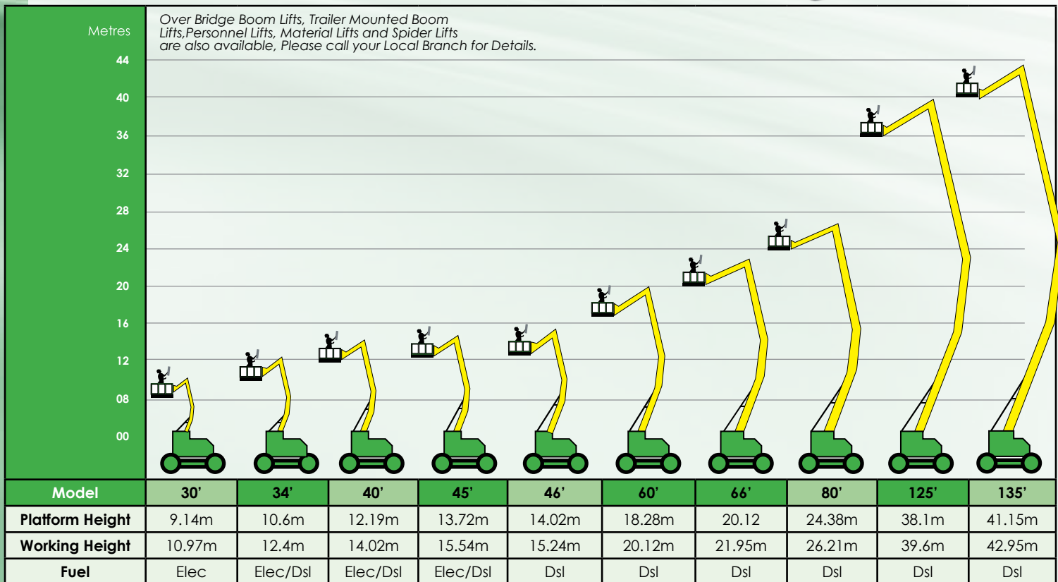
Boom Lifts: Knuckle
